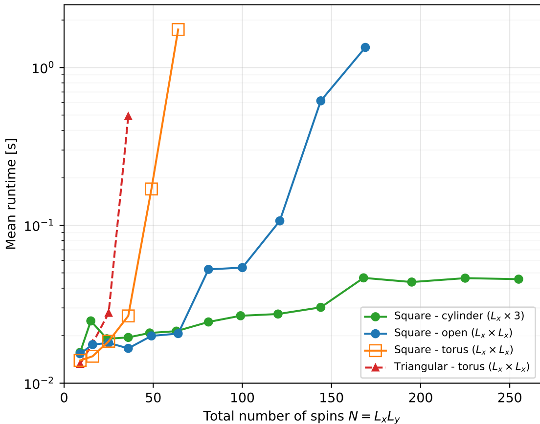
Runtime for Z using DPMC
